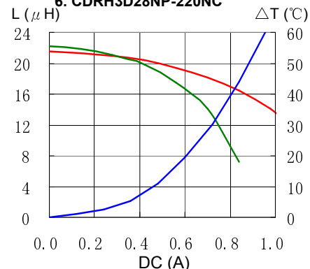
6. CDRH3D28NP-220NC
