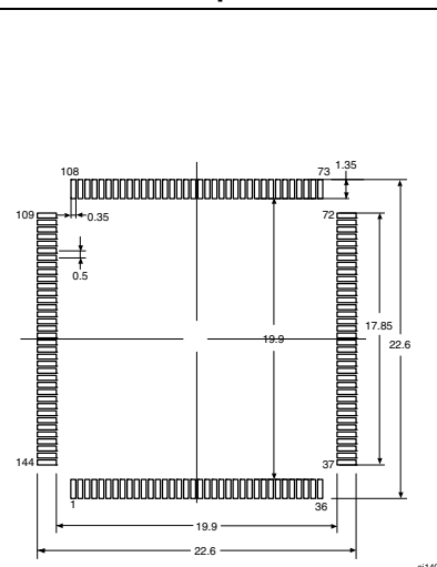
Figure 64. Recommended footprint (1)(2)
