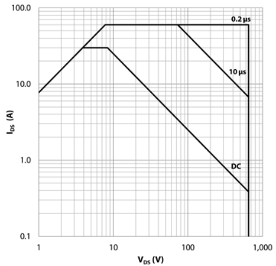
Figure 12: Safe Operating Area @ T_{case} = 25\text{ °C}
