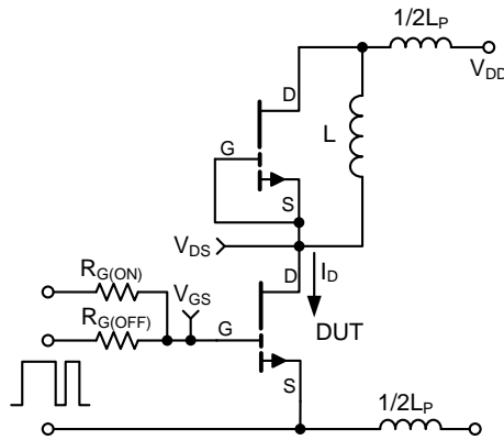
Figure 16: GS66508P Switching Loss Test Circuit
