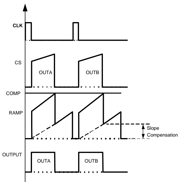
Figure 19. Timing Diagram for Current Mode Configuration
