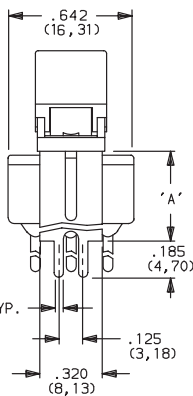
SNAP-IN
