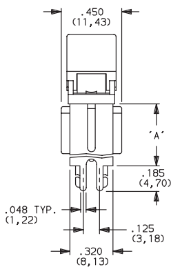
SNAP-IN
