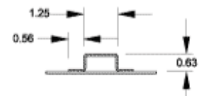
Section Z-Z
