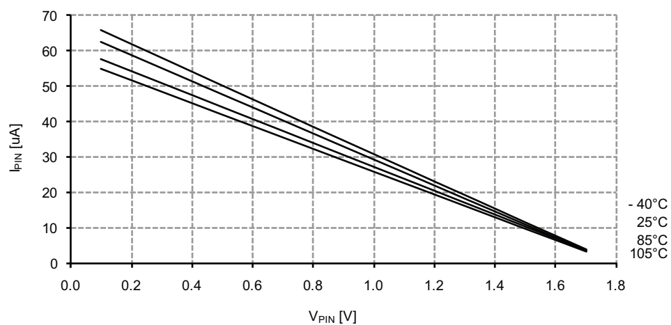
Figure 37-189. I/O pin pull-up resistor current vs. input voltage.
