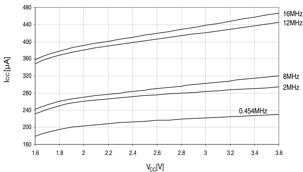
Figure 37-272. Standby supply current vs. V_{CC} .
