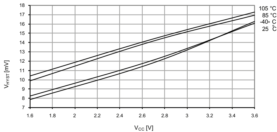
Figure 37-136. Analog comparator hysteresis vs. V_{CC} . High-speed, small hysteresis.
