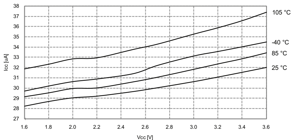
Figure 37-262. Idle mode supply current vs. V_{\text{CC}} .
