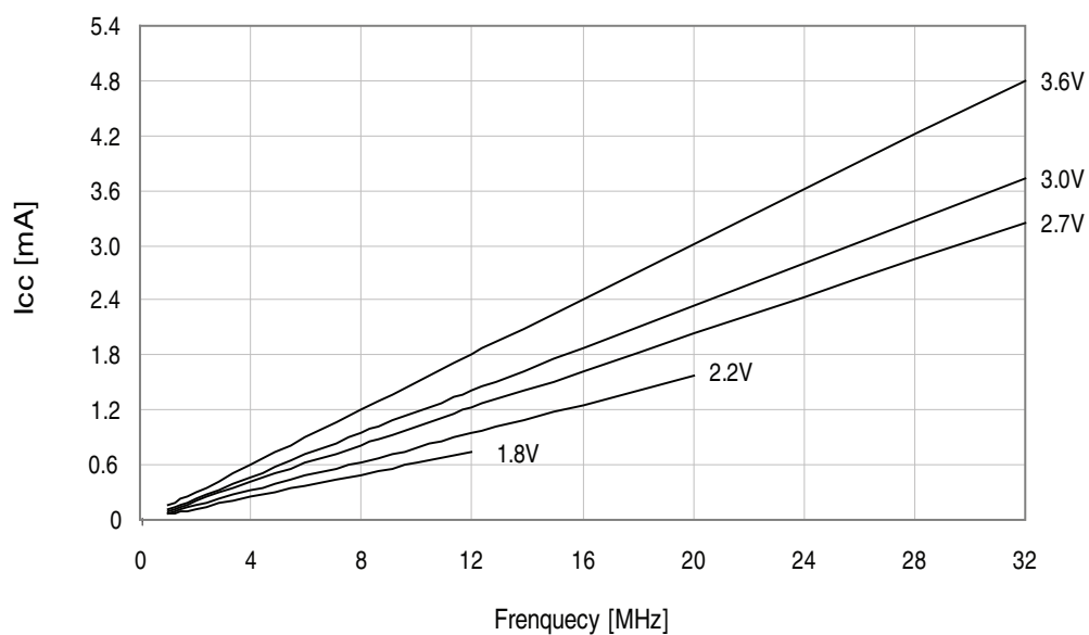
Figure 37-261. Idle mode supply current vs. frequency.
