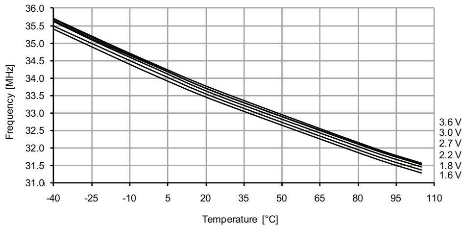
Figure 37-76. 32MHz internal oscillator frequency vs. temperature. DPLL disabled.
