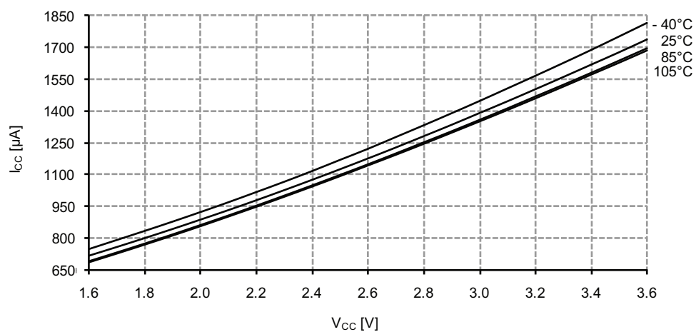
Figure 37-182. Idle mode current vs. V_{CC} .
