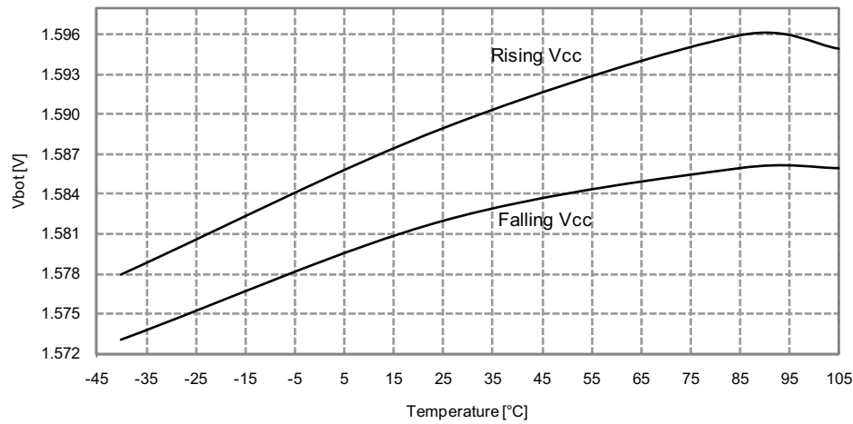
Figure 37-312. BOD thresholds vs. temperature. BOD level = 1.6V
