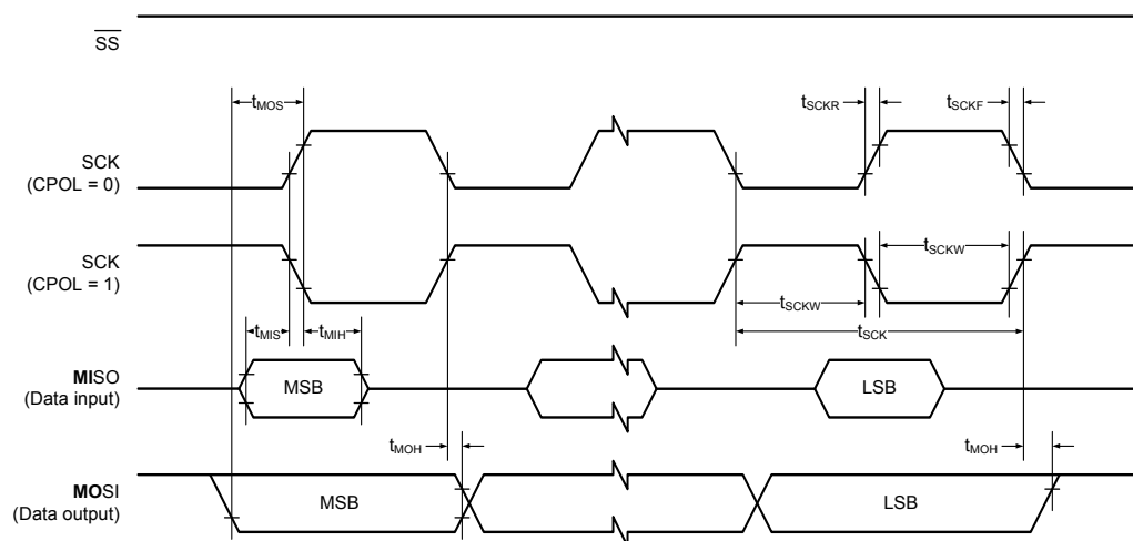
Figure 36-19. SPI timing requirements in master mode.
