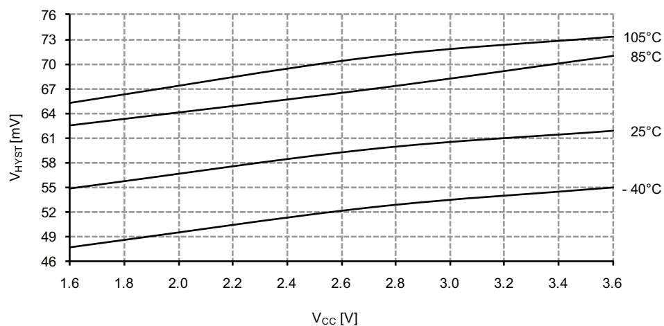
Figure 37-223. Analog comparator hysteresis vs. V_{CC} . Low power, large hysteresis.
