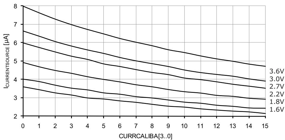
Figure 37-224. Analog comparator current source vs. calibration value. Temperature = 25°C.
