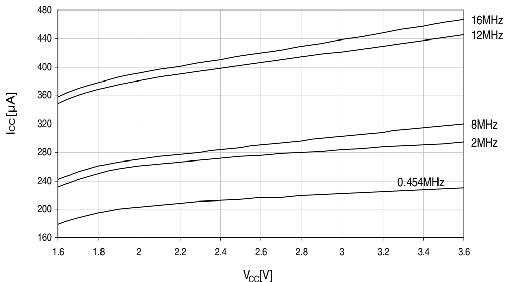
Figure 37-20. Standby supply current vs. V_{CC} .
