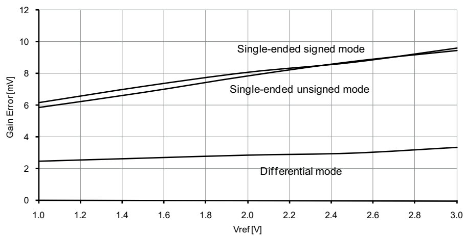
Figure 37-210. Gain error vs. V_{REF} . T = 25^{\circ}\text{C} , V_{CC} = 3.6\text{V} , ADC sampling speed = 500ksps.
