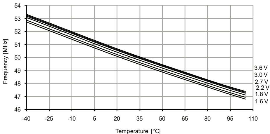
Figure 37-164. 48MHz internal oscillator frequency vs. temperature.
