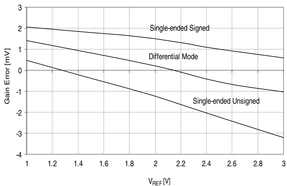
Figure 37-294. Gain error vs. V_{REF} T = 25^{\circ}\text{C} , V_{CC} = 3.6\text{V} , ADC sampling speed = 500ksps
