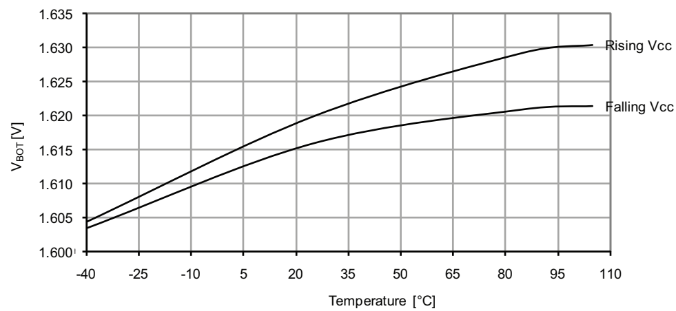
Figure 37-144. BOD thresholds vs. temperature.
