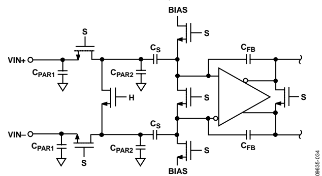
Figure 26. Switched-Capacitor Input
