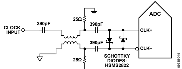
Figure 33. Balun-Coupled Differential Clock (Up to 625 MHz)
