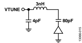
Figure 6. VTUNE Interface
