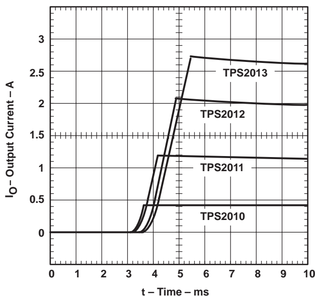
Figure 30. Turned-On (Enabled) Into Short Circuit, V_{I(IN)} = 5.5 V
