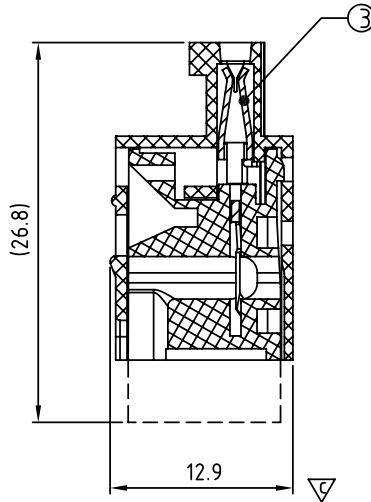
SECTION P-P
