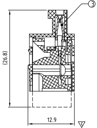
SECTION P-P
