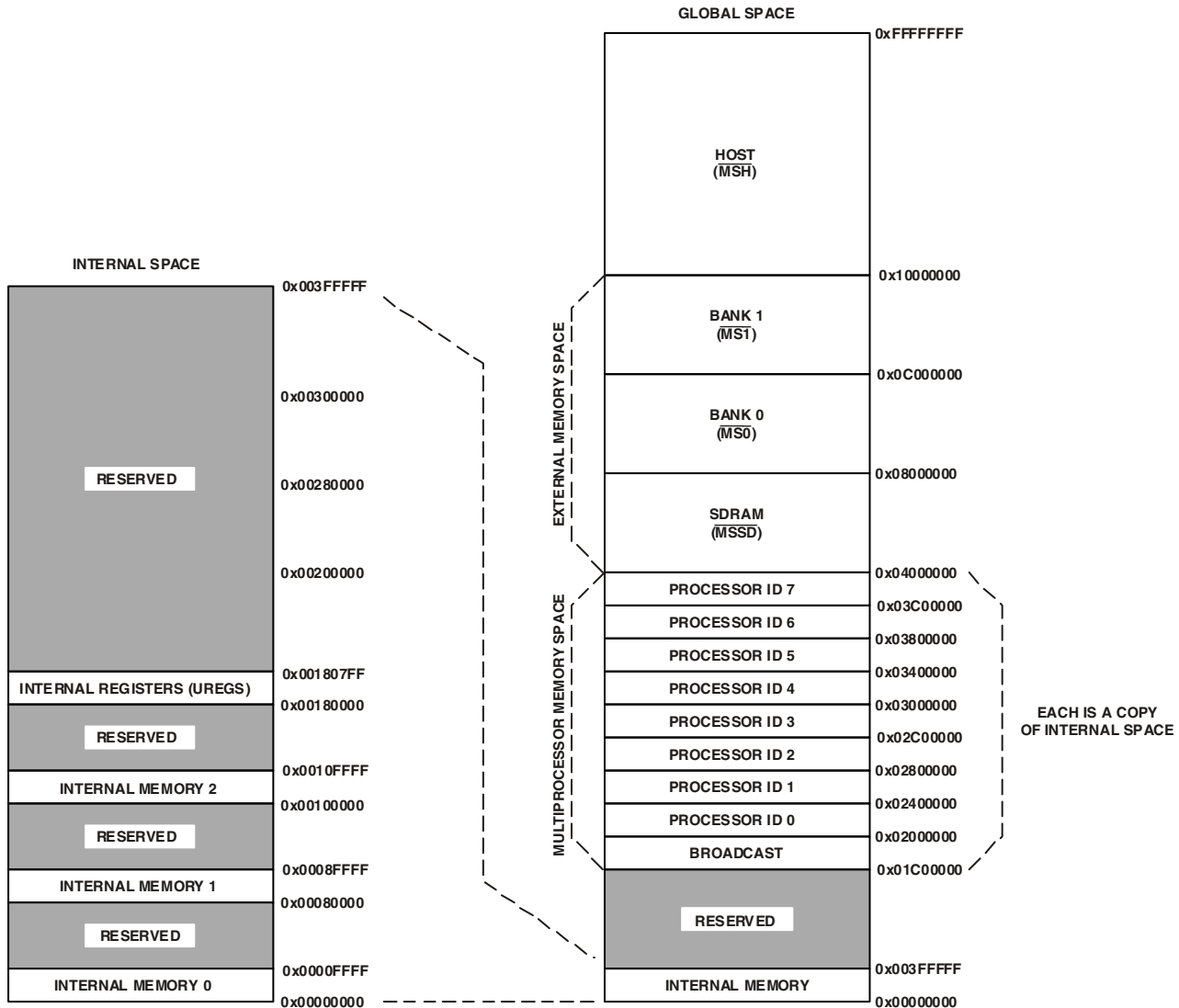
Figure 3. Memory Map
