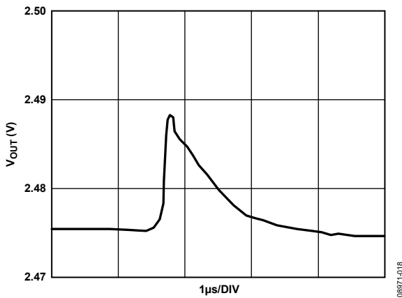
Figure 18. Major-Code Transition Glitch Energy
