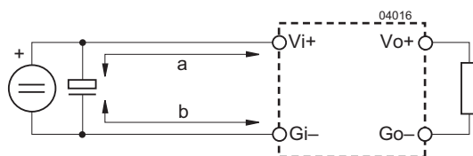
Fig. 3 Switching regulator with long supply lines.
