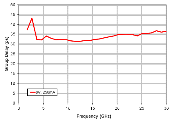
Group Delay
