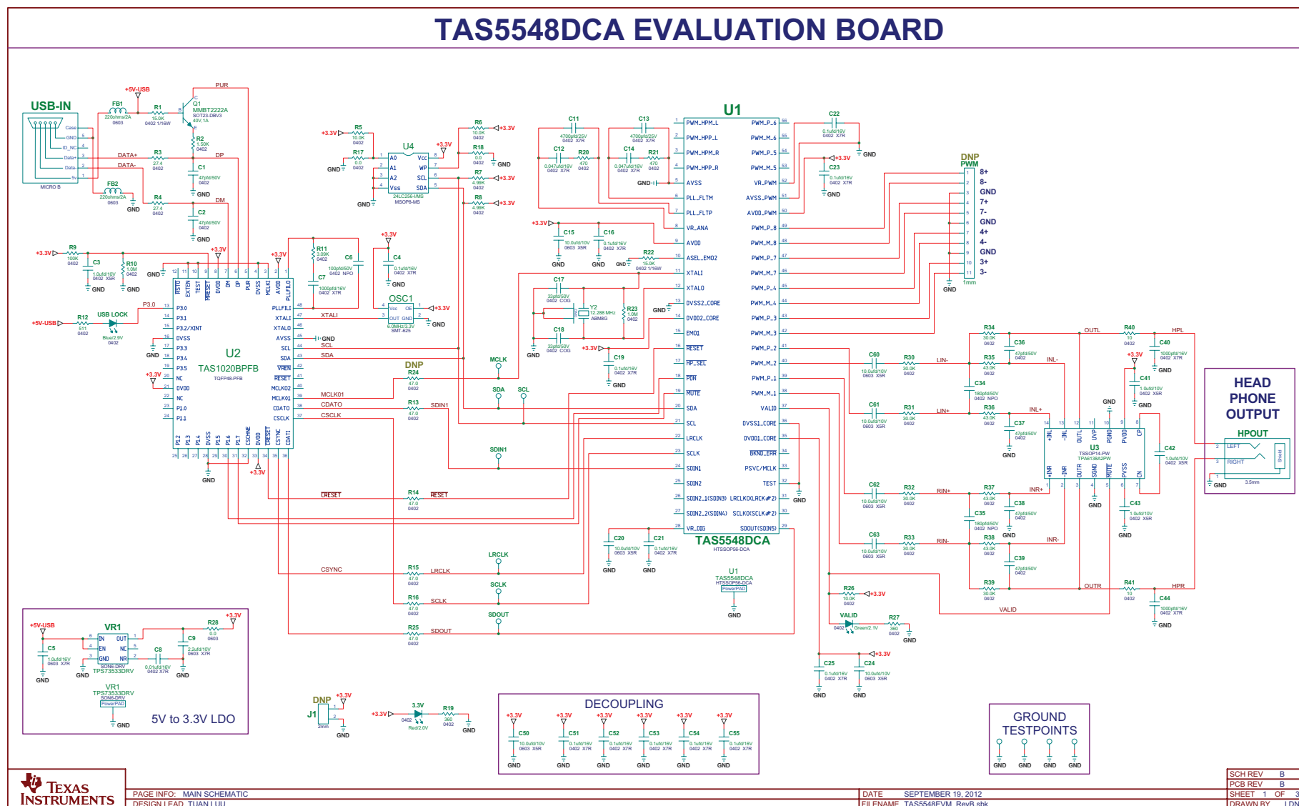
Figure 11. TAS5548EVM Schematic
