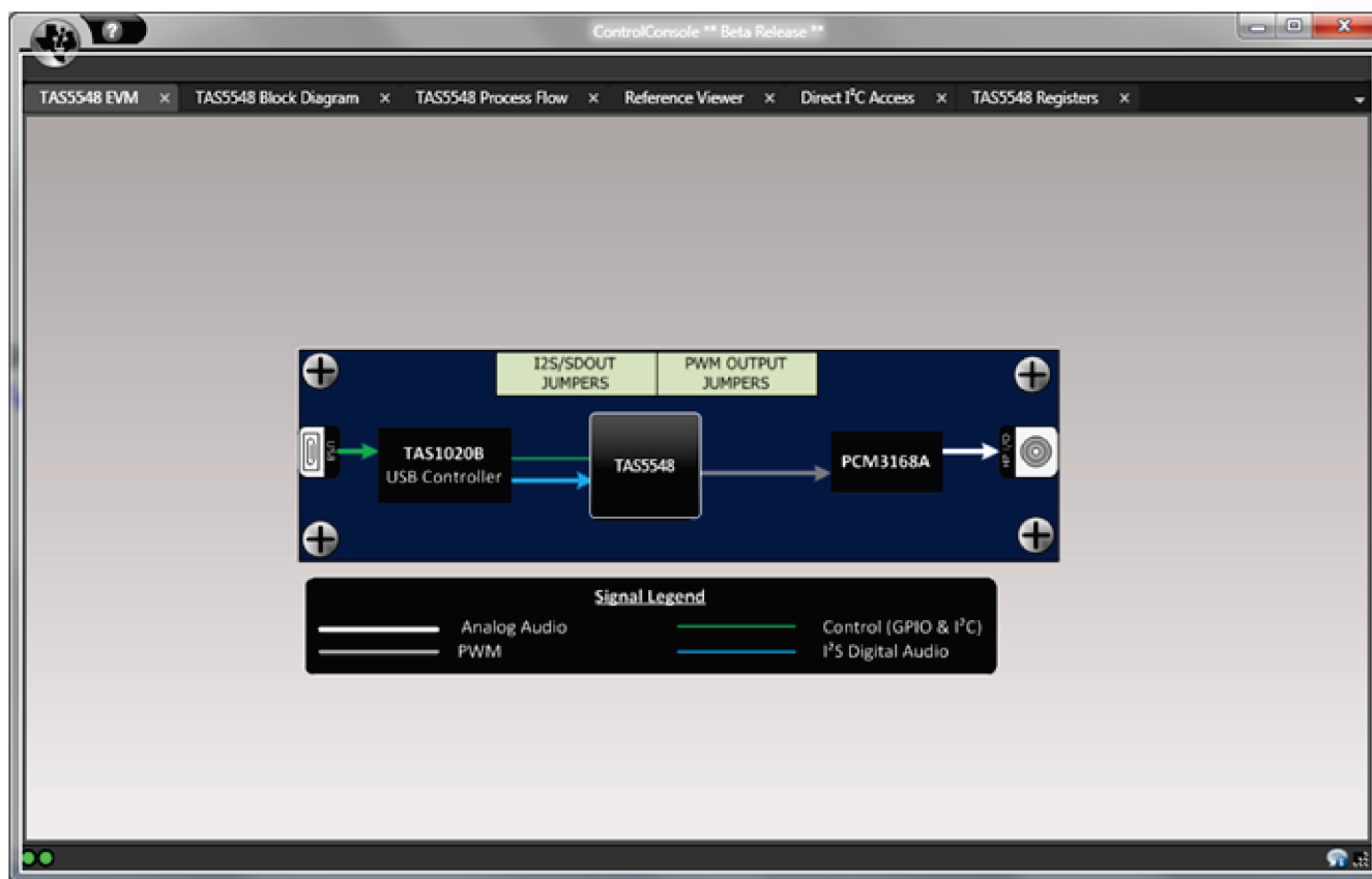
Figure 5. Main Tab
