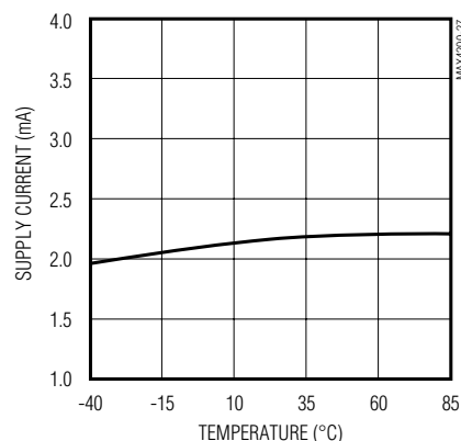
SUPPLY CURRENT (PER BUFFER) vs. TEMPERATURE
