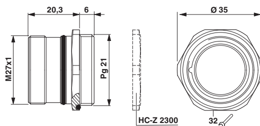
Dimensional drawing
