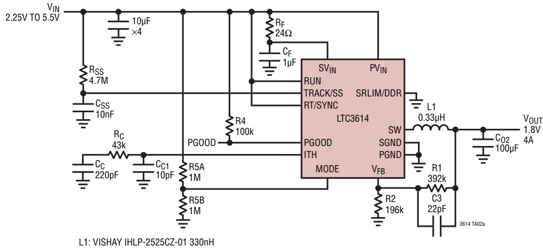
General Purpose Buck Regulator with Fast Compensation and Improved Step Response, 2.25MHz
