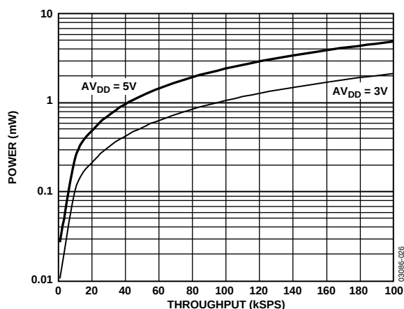
Figure 26. Power vs. Throughput Rate
