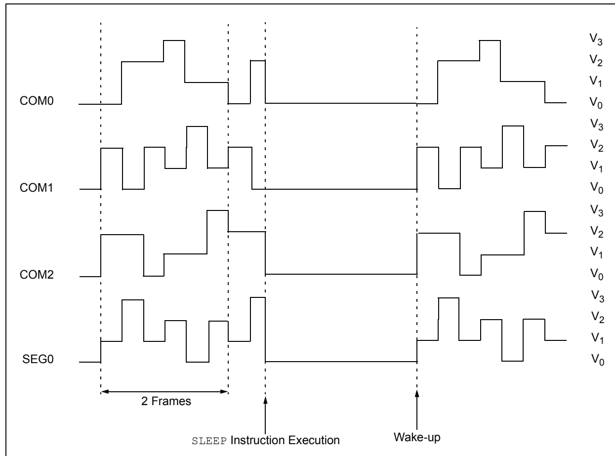
FIGURE 27-20: SLEEP ENTRY/EXIT WHEN SLPEN = 1
