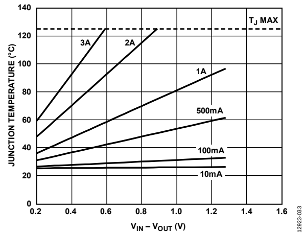
Figure 35. 6400 mm 2 of PCB Copper, T_A = 25^\circ\text{C}
