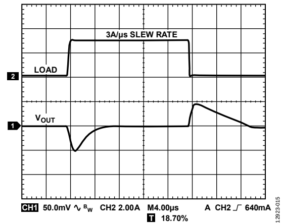
Figure 15. Load Transient Response, C_{OUT} = 47\text{ }\mu\text{F} , V_{IN} = 1.8\text{ V} , V_{OUT} = 1.3\text{ V}
