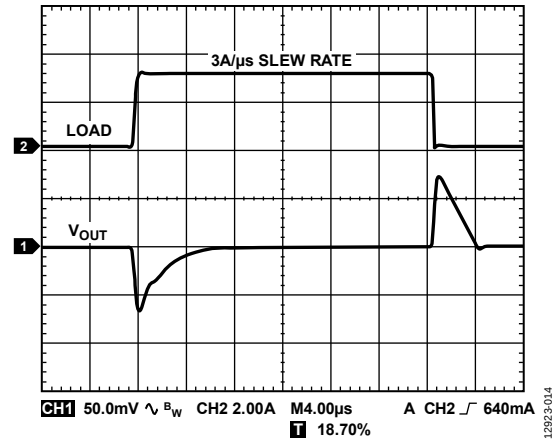
Figure 14. Load Transient Response, C_{OUT} = 10\text{ }\mu\text{F} , V_{IN} = 1.8\text{ V} , V_{OUT} = 1.3\text{ V}
