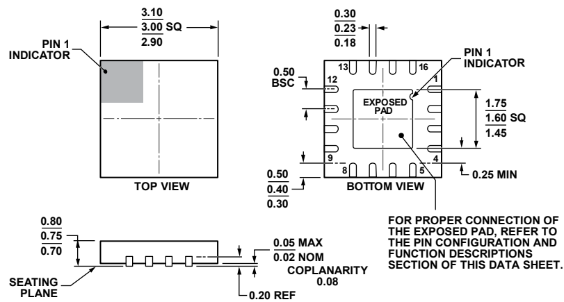
Figure 49. 16-Lead Lead Frame Chip Scale Package [LFCSP] 3 mm × 3 mm Body and 0.75 mm Package Height (CP-16-22)
