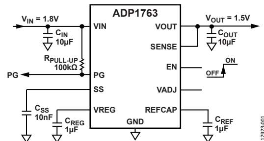
Figure 1. Fixed Output Operation
