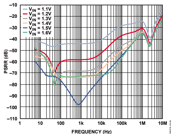
Figure 19. Power Supply Rejection Ratio (PSRR) vs. Frequency for Various Loads, V_{OUT} = 0.9 V, Load Current = 3 A
