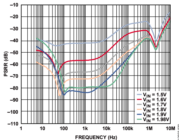
Figure 20. Power Supply Rejection Ratio (PSRR) vs. Frequency for Various Loads, V_{OUT} = 1.3 V, Load Current = 3 A
