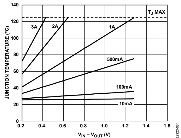
Figure 36. 500 mm 2 of PCB Copper, T_A = 25^\circ\text{C}
