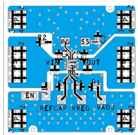
Figure 47. Typical Board Layout, Top Side
