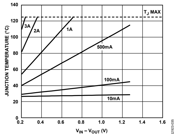
Figure 37. 25 mm 2 of PCB Copper, T_A = 25^\circ\text{C}
