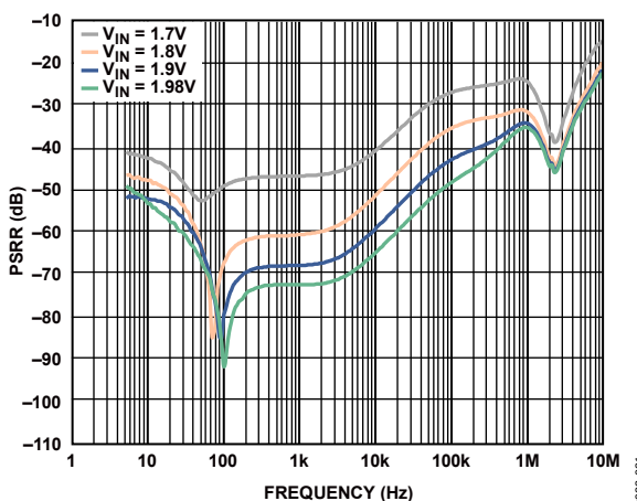
Figure 21. Power Supply Rejection Ratio (PSRR) vs. Frequency for Various Loads, V_{OUT} = 1.5 V, Load Current = 3 A
