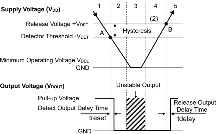
Operation Diagram
