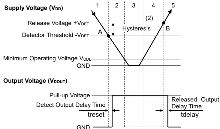
Operation Diagram
