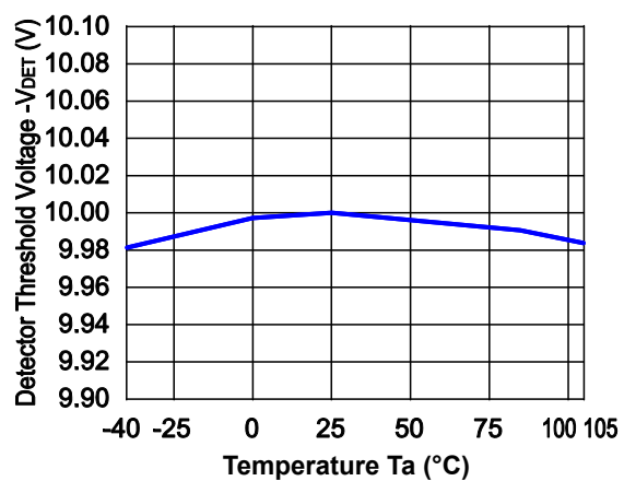
R3150NxxxA/B (-V DET = 10.0 V)
