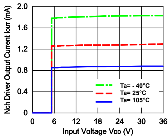
R3150NxxxB (+V DET = 5.3 V, V DOUT = 0.05 V)
