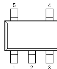
SOT-23-5 Pin Configurations
