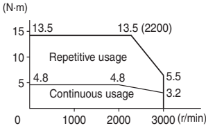
R88M-G1K020T (1 kW)
