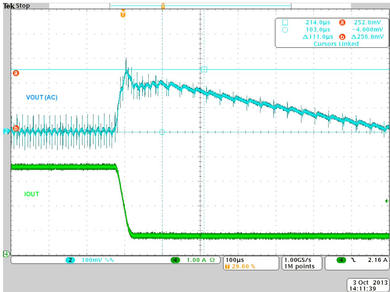
Figure 22. Load step-down from 100% to 20% I_{\text{OUT}} , V_{\text{IN}} = 115 \text{ V}_{\text{AC}} , V_{\text{OUT\_OVERSHOOT}} = 256 \text{ mV}
