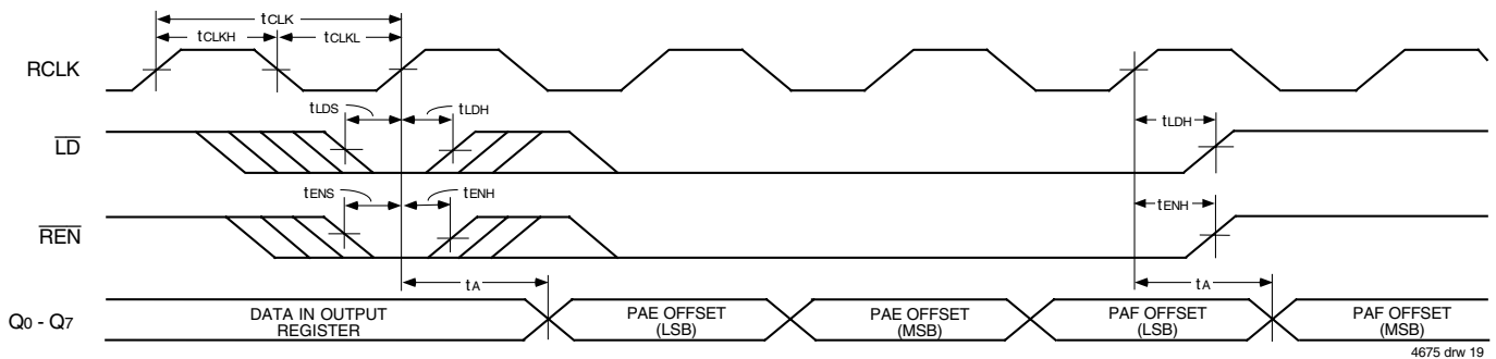
Figure 16. Parallel Read of Programmable Flag Registers (IDT Standard and FWFT Modes) for the IDT72281
