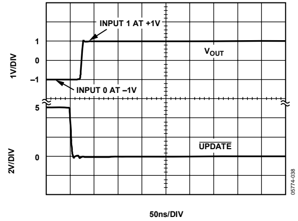
Figure 37. AD8106 Switching Time
