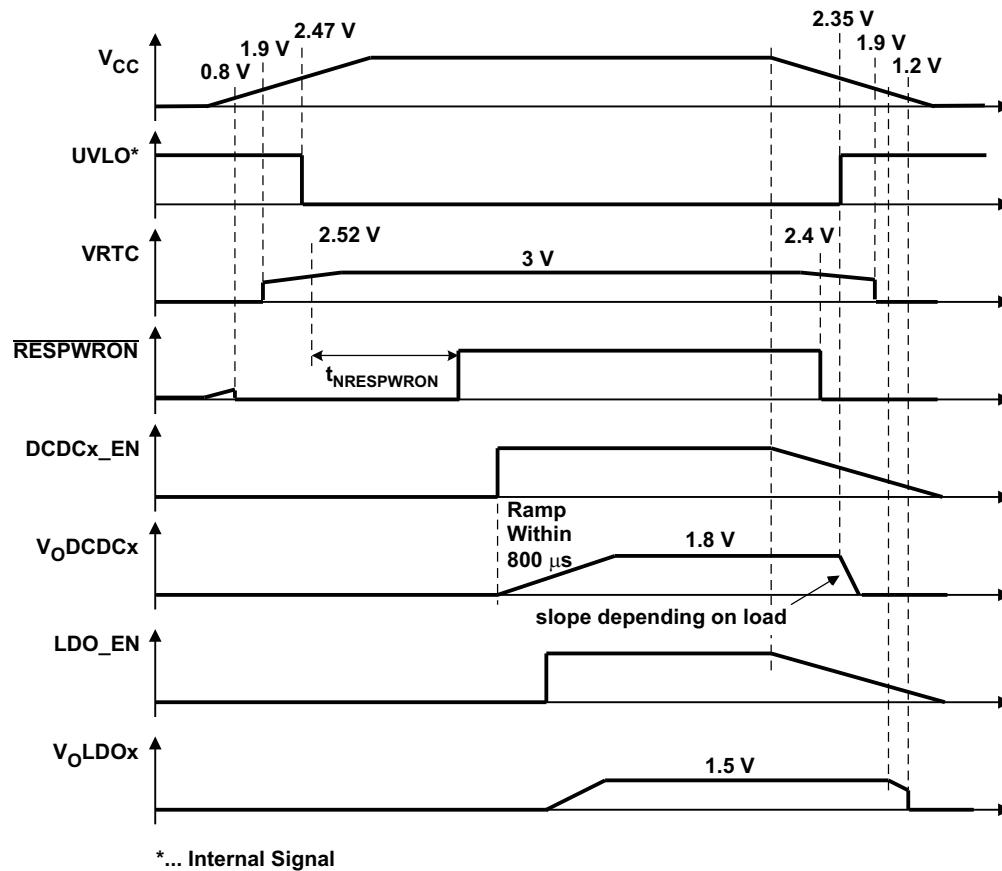
Figure 27. Power-Up and Power-Down Timing
