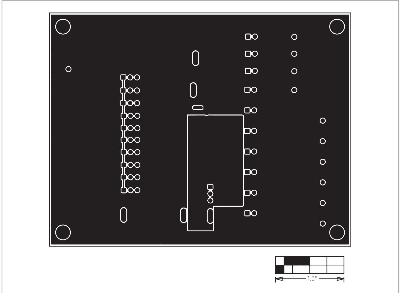
Figure 4. MAX17108 EV Kit PCB Layout—Solder Side
