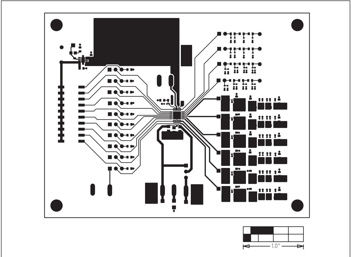
Figure 3. MAX17108 EV Kit PCB Layout—Component Side
