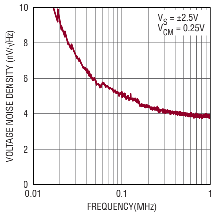
Input Referred Voltage Noise Density
