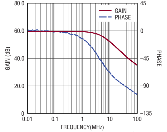
Gain/Phase vs Frequency
