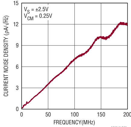
Input Referred Current Noise
