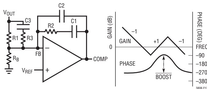
Figure 12. Type 3 Amplifier Compensation
