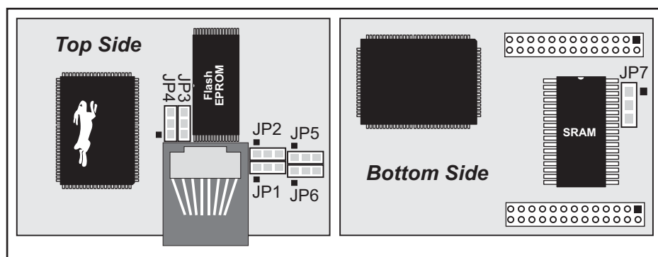
Figure A-5. Location of RCM2200 Configurable Positions
