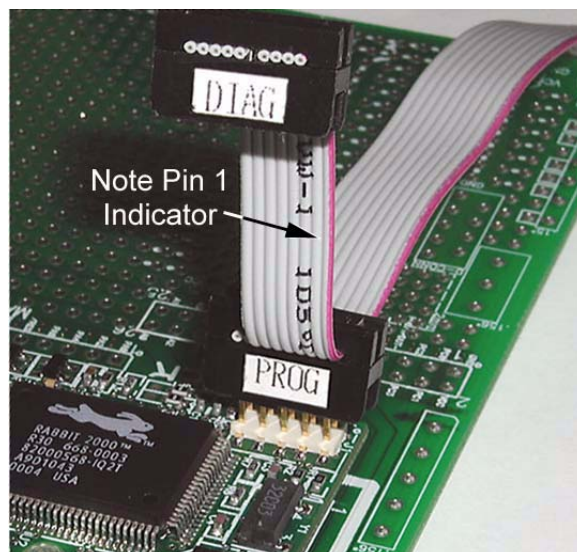
Figure 2. Connect Programming Cable to RCM2200
