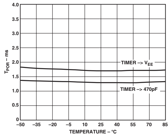
TPC 19. POR Delay vs. Temperature
