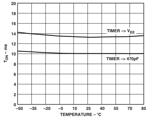
TPC 21. Maximum Current Limit On Time vs. Temperature
