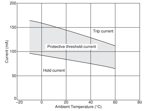
PTGL07AR750M7B52B0
