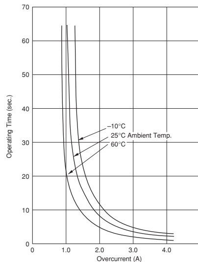
PTGL12AR1R2H2B51B0
