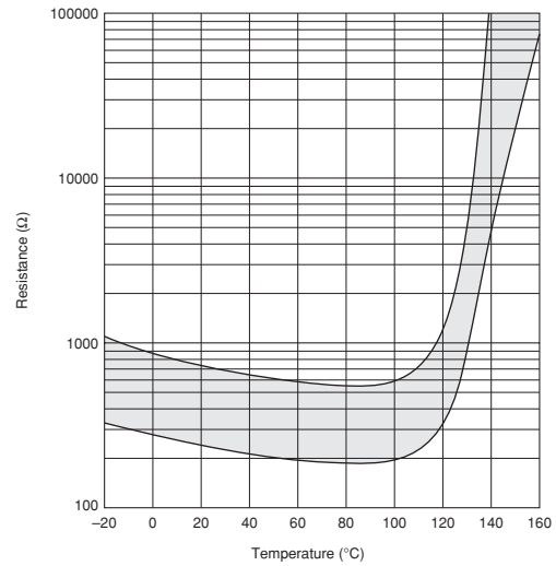
PRF18/21AR471Q Type
