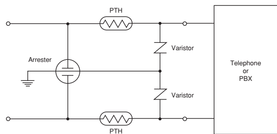
(5) Telecommunication Circuit
