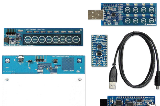
LC717A30UJ Evaluation Kit
