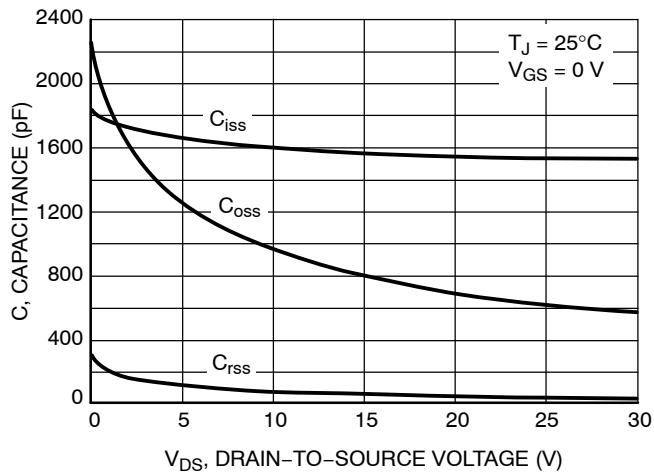
Figure 17. Capacitance Variation
